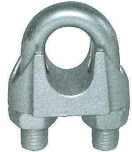
GALVANISED AND STAINLESS STEEL MALLEABLE CAST ROPE CLAMPS (COMMERCIAL TYPE) TO DIN741
